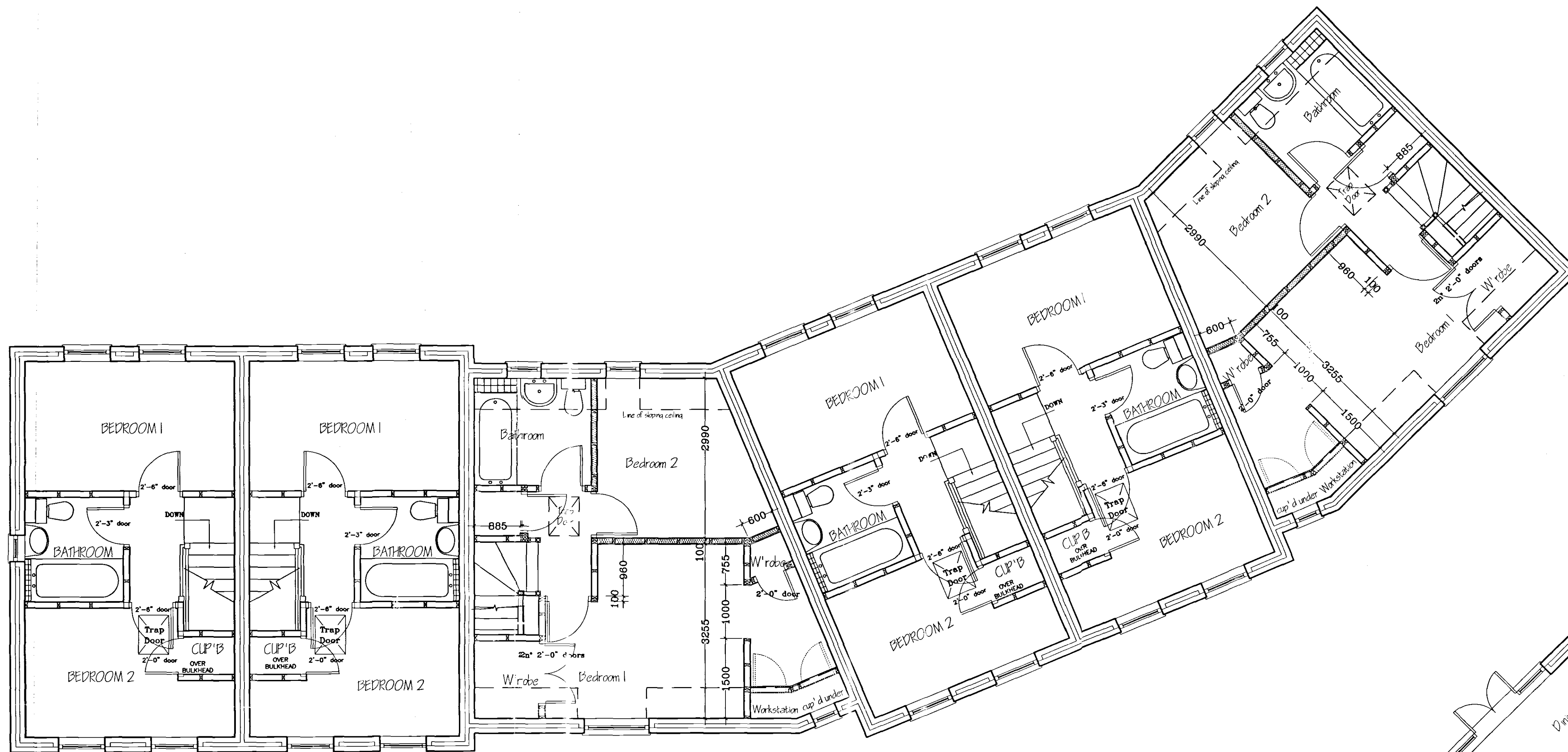
FIRST FLOOR LAYOUT
