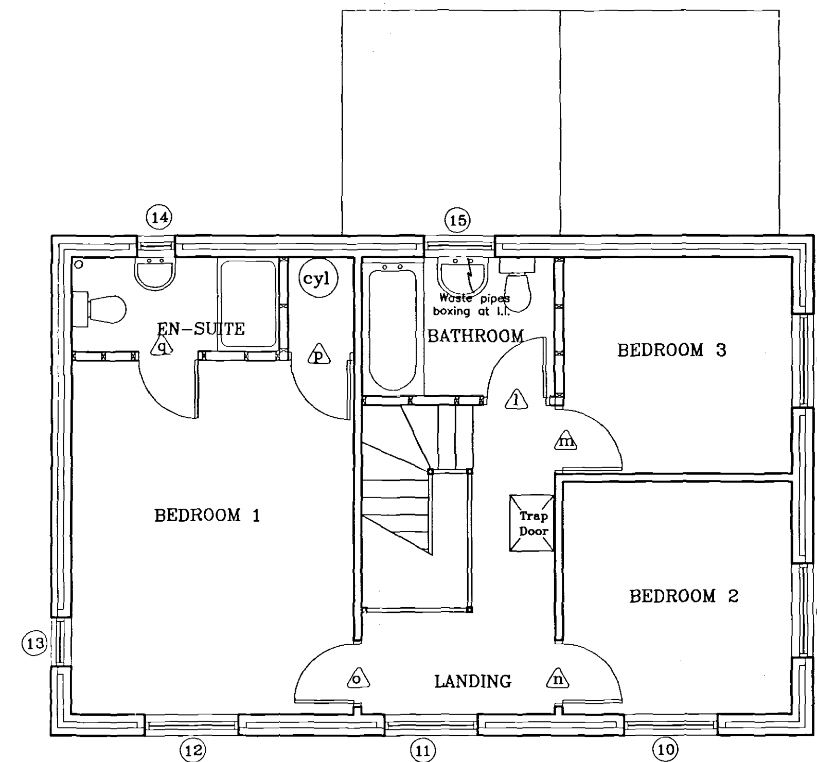
FIRST FLOOR LAYOUT
