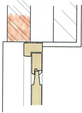
jamb section entrance door
