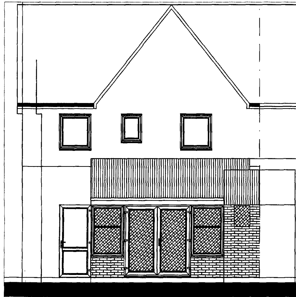
PROPOSED REAR ELEVATION 1:50
