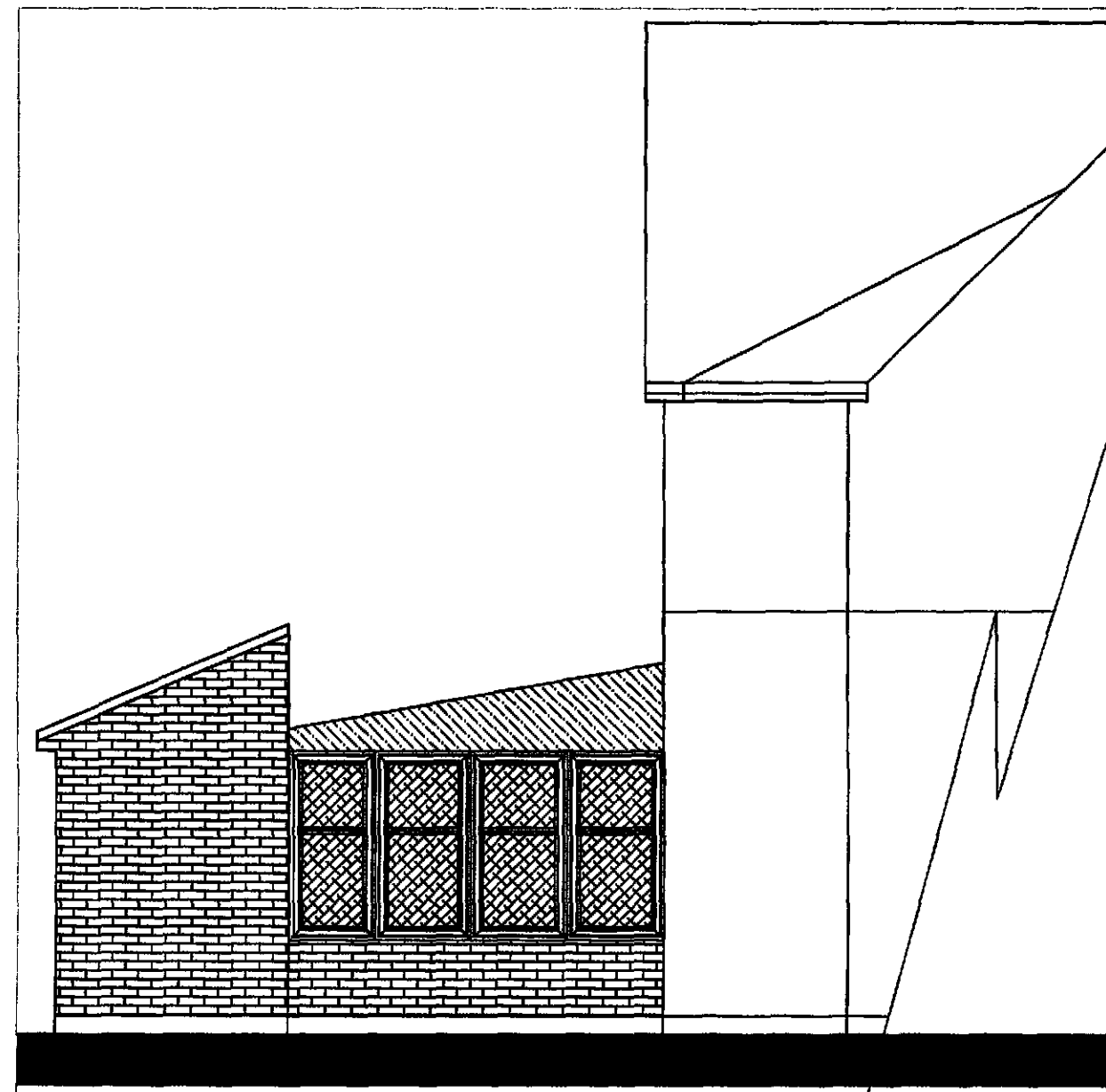
PROPOSED SIDE ELEVATION 1:50
