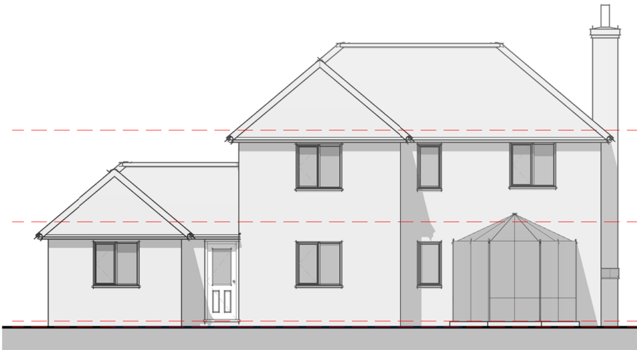
Elevation 03 - Rear 1 : 100
