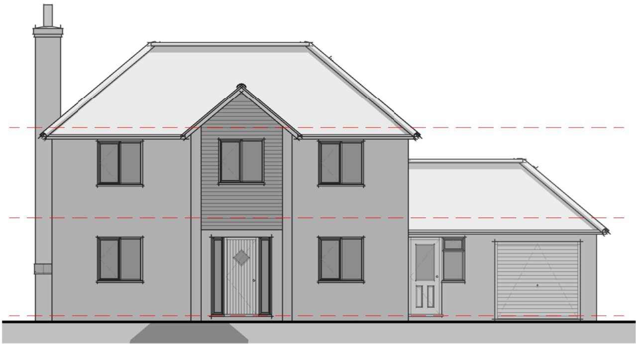
Elevation 01 - Front 1 : 100
