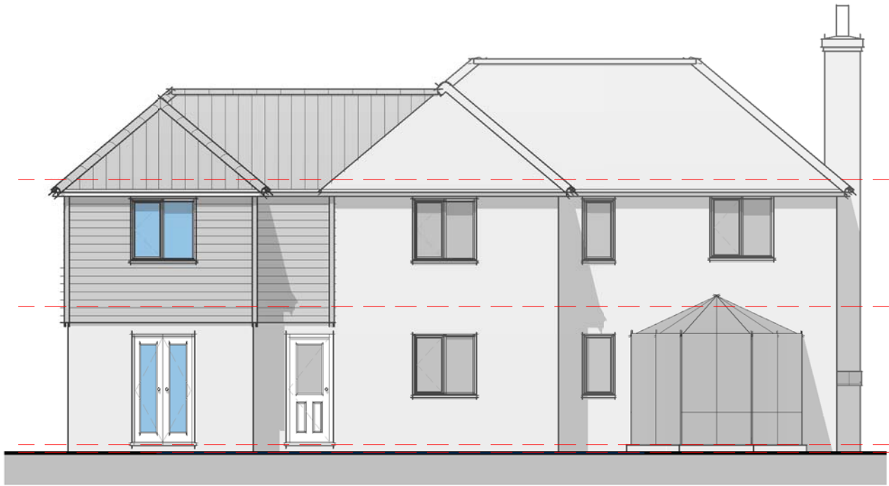
Elevation 03 - Rear 1 : 100
