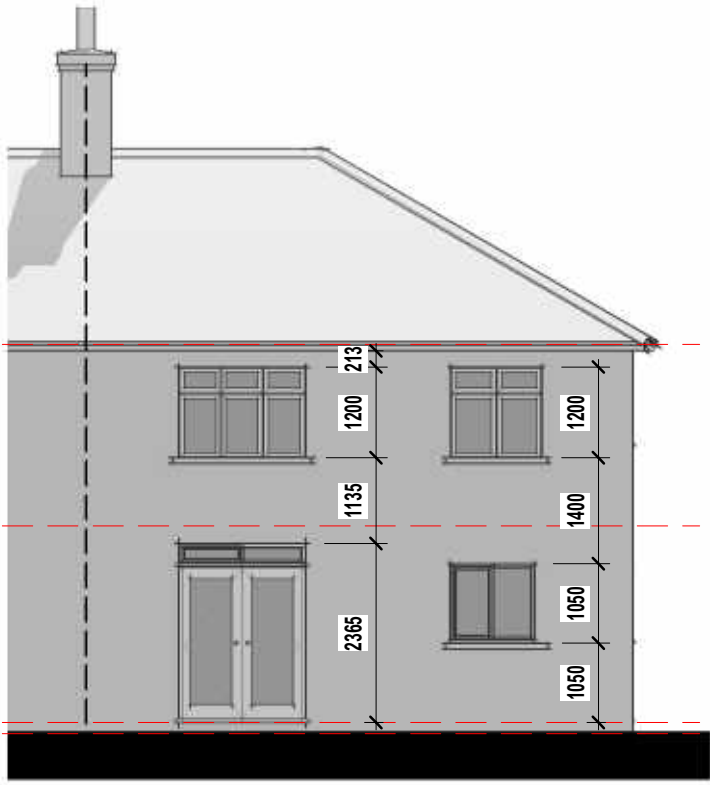
Elevation 03 - Rear 1 : 100
