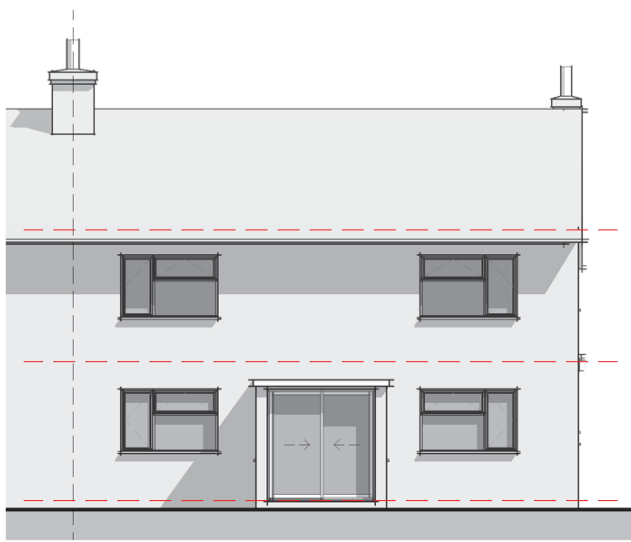
Elevation 01 – Front
