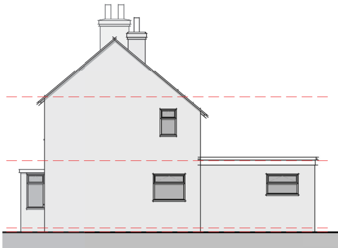
Elevation 02 – Right
