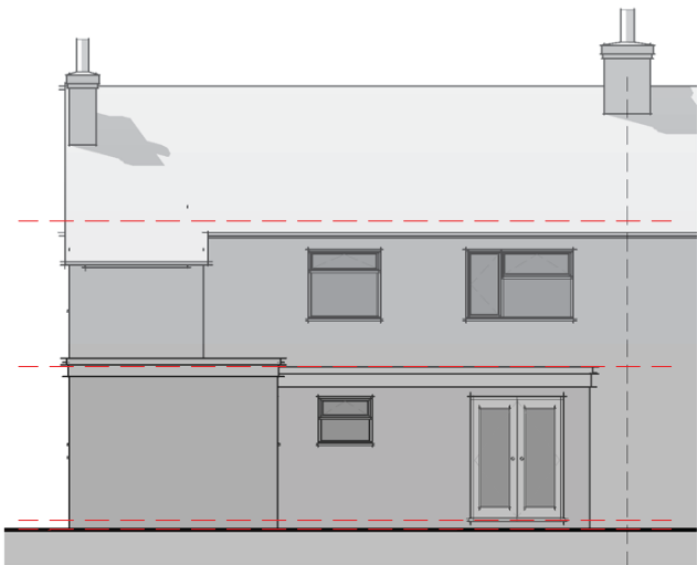
Elevation 03 – Rear
