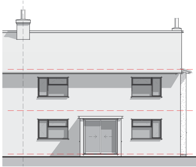
Elevation 01 – Front 1 : 100
