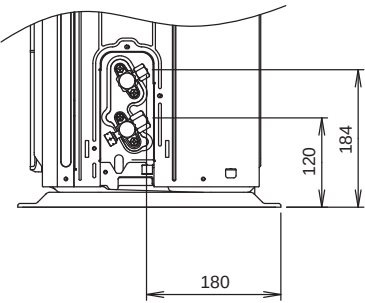
Side view (Bulb part)
