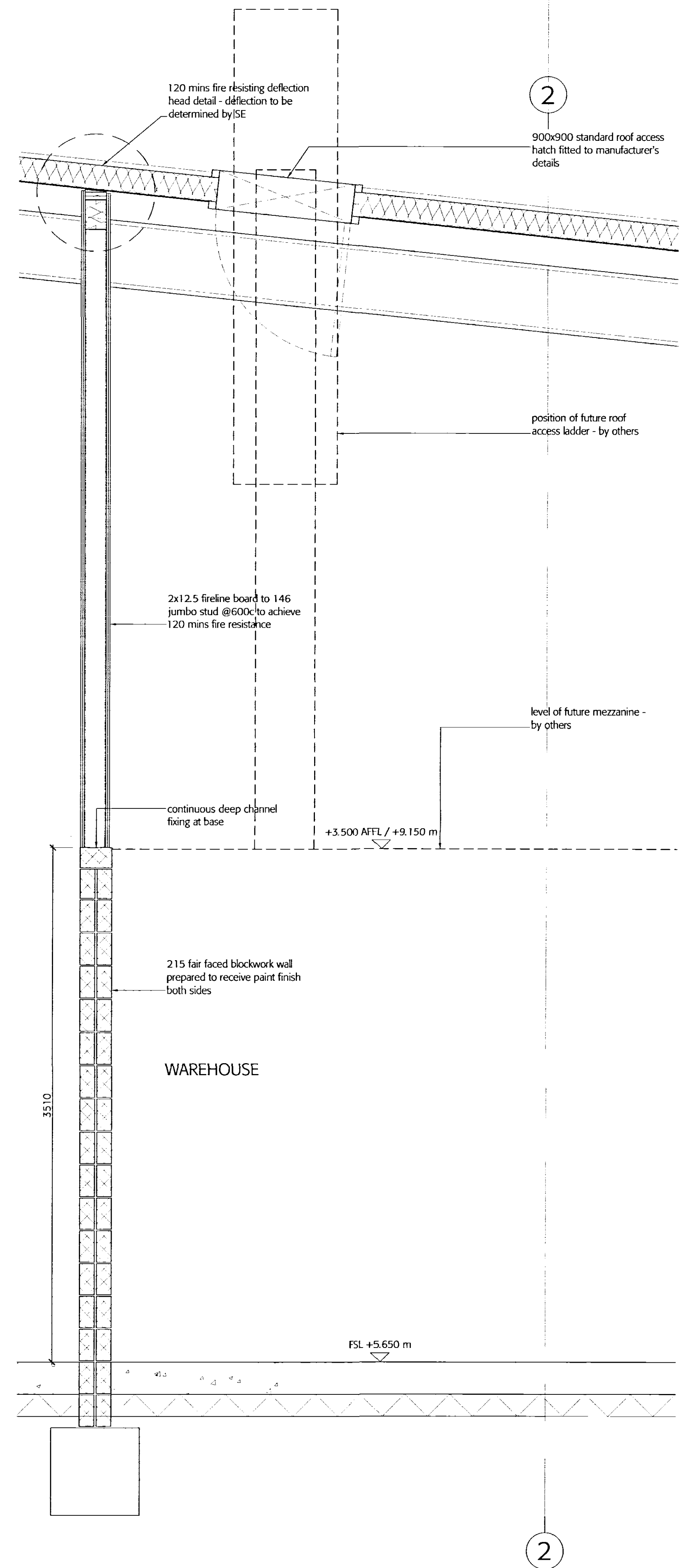
C_06 section through fire wall
