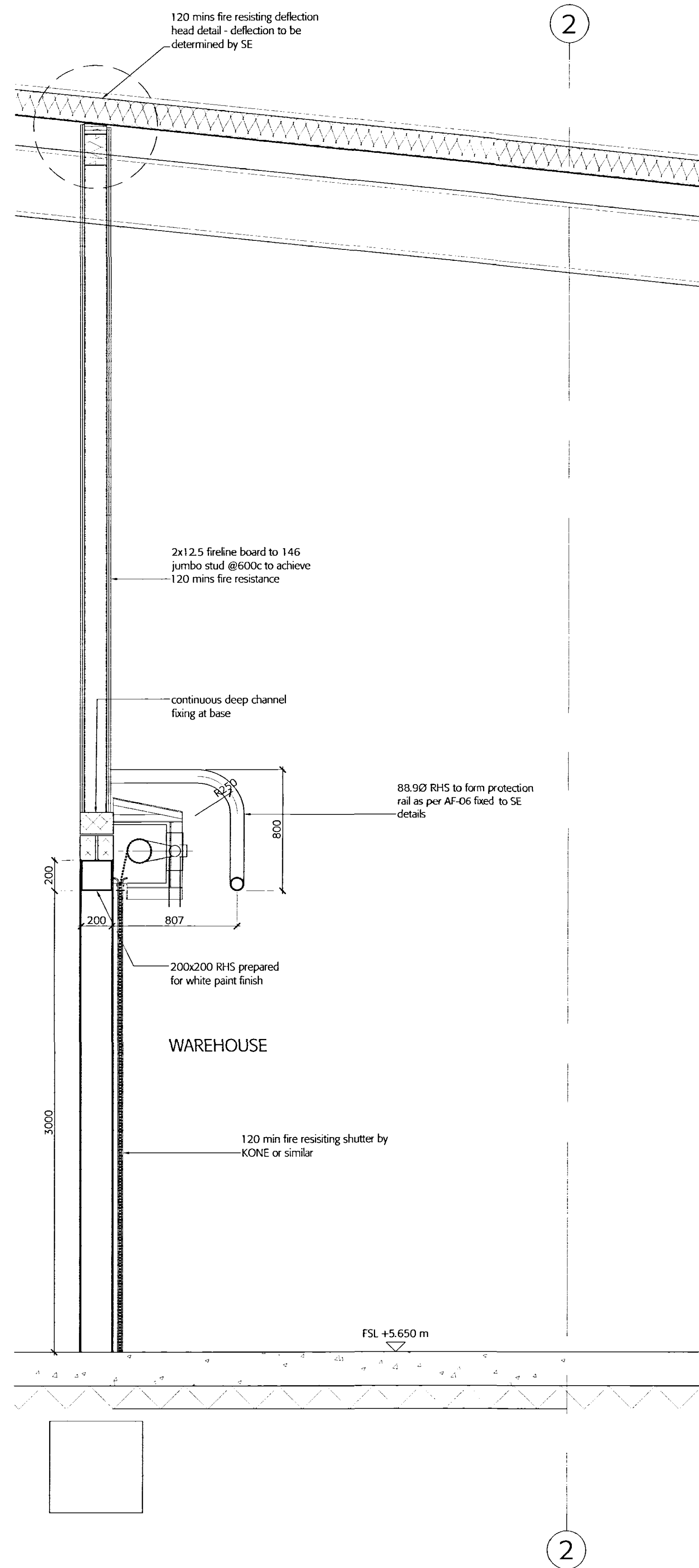
C_05 section through fire shutter
