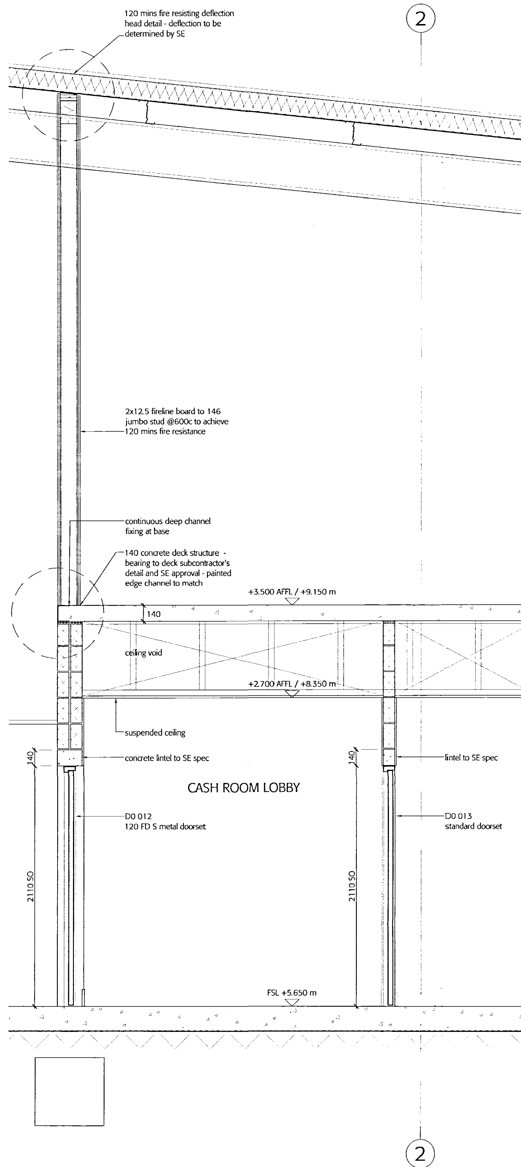
C_04 section through office - showing typical door conditions
