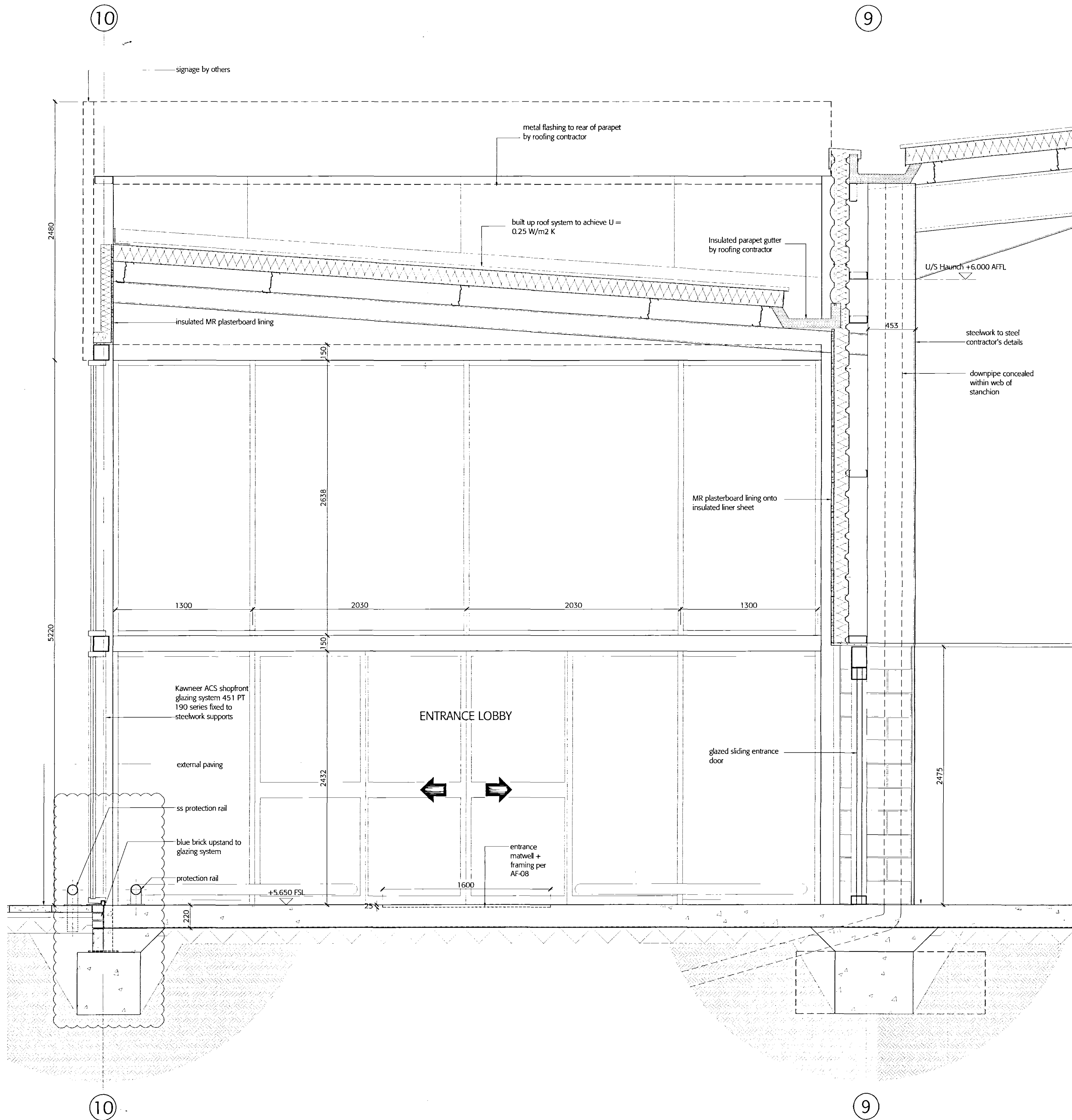
C_04 section through glazed entrance lobby
