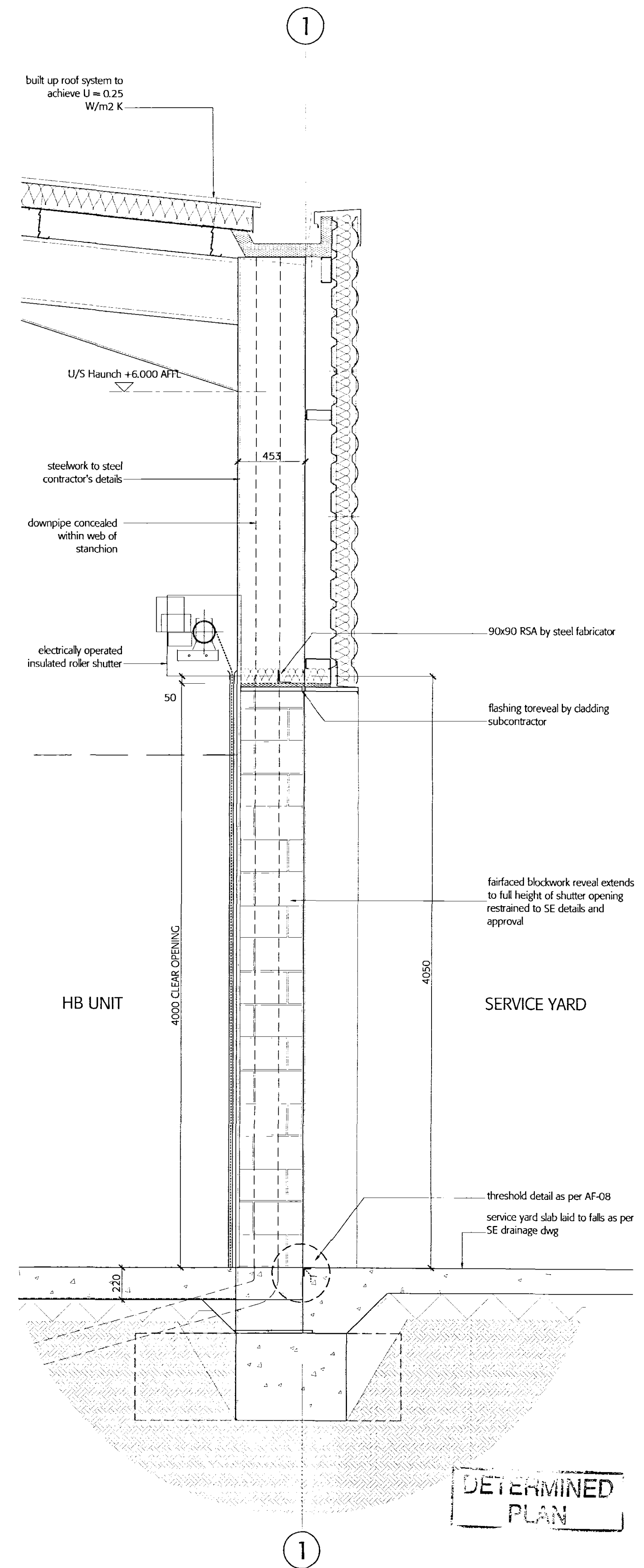
C_05 section through loading bay door opening
