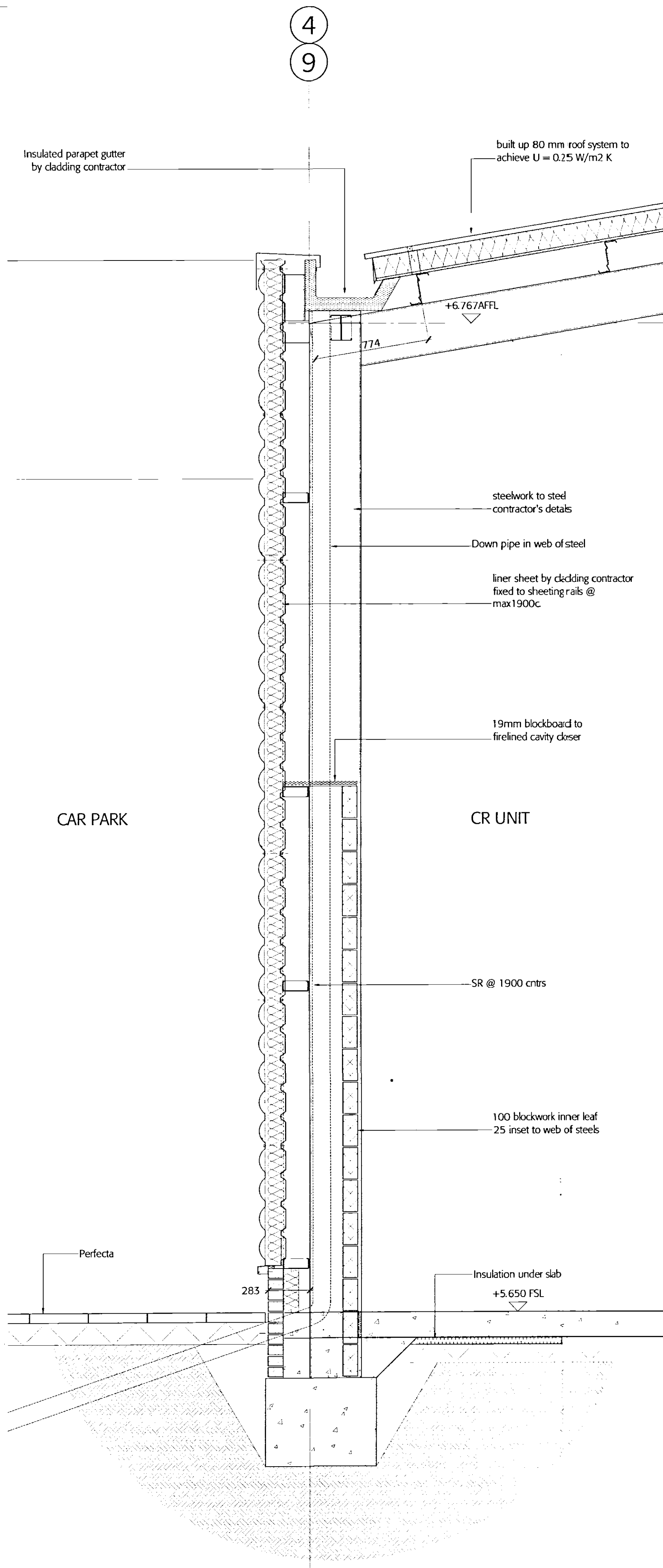
B_01 section through typical wall construction to CR unit
