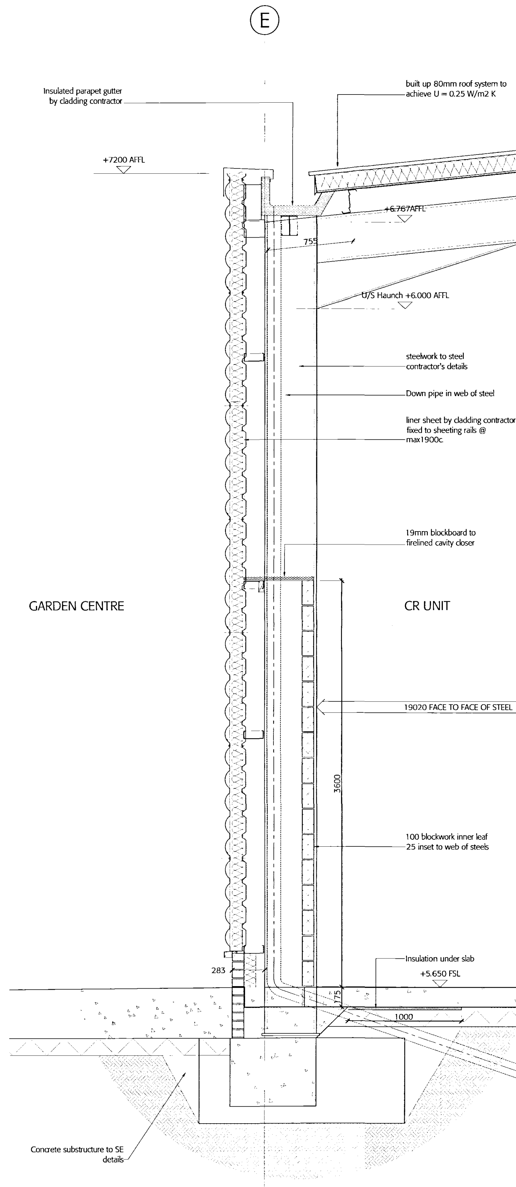
B_02 section through typical wall to garden centre
