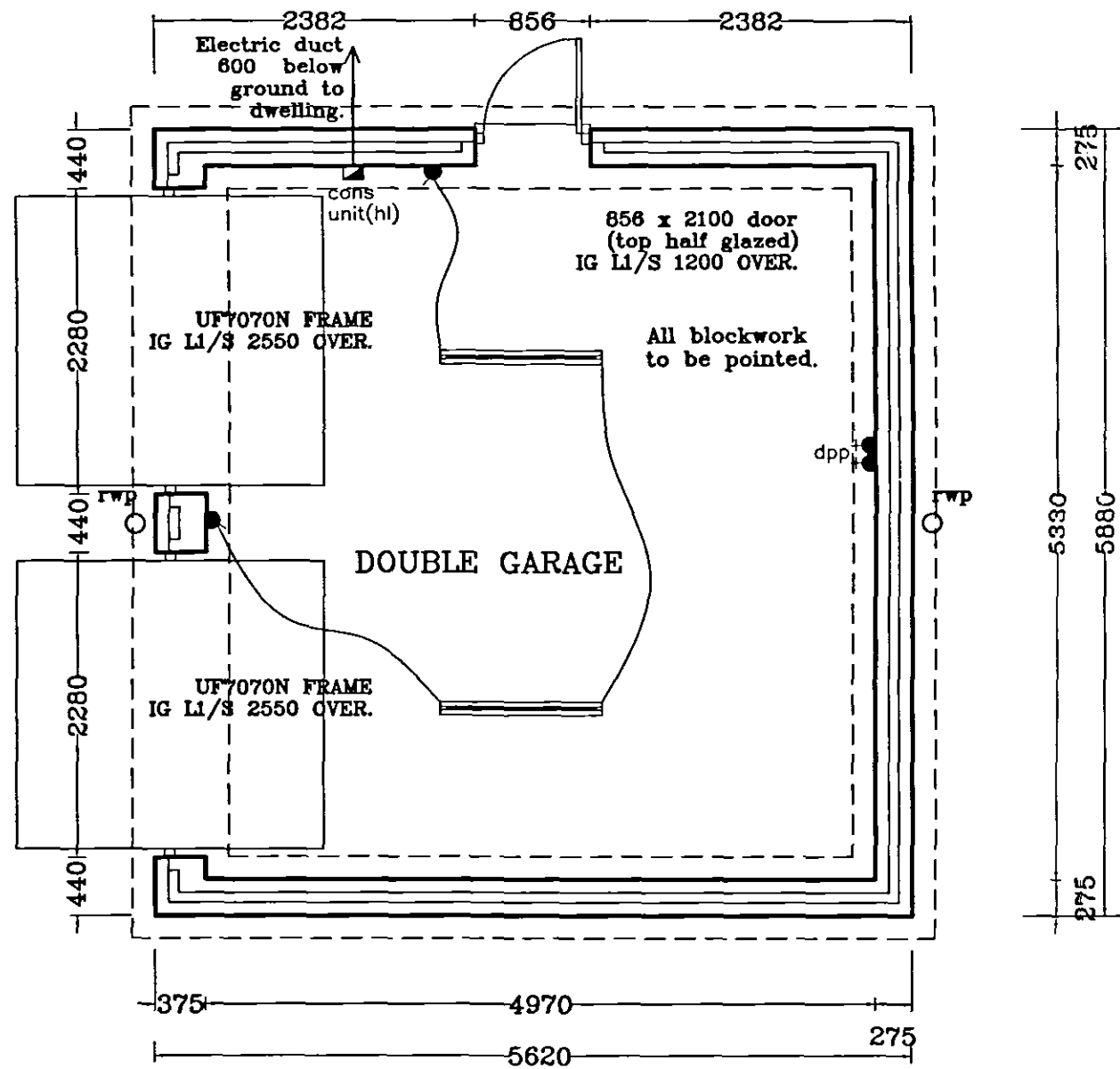
FLOOR LAYOUT
