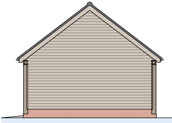
North Elevation
