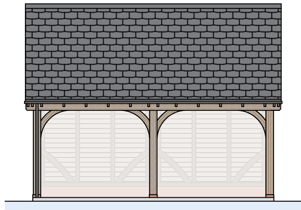
West Elevation 1:100
