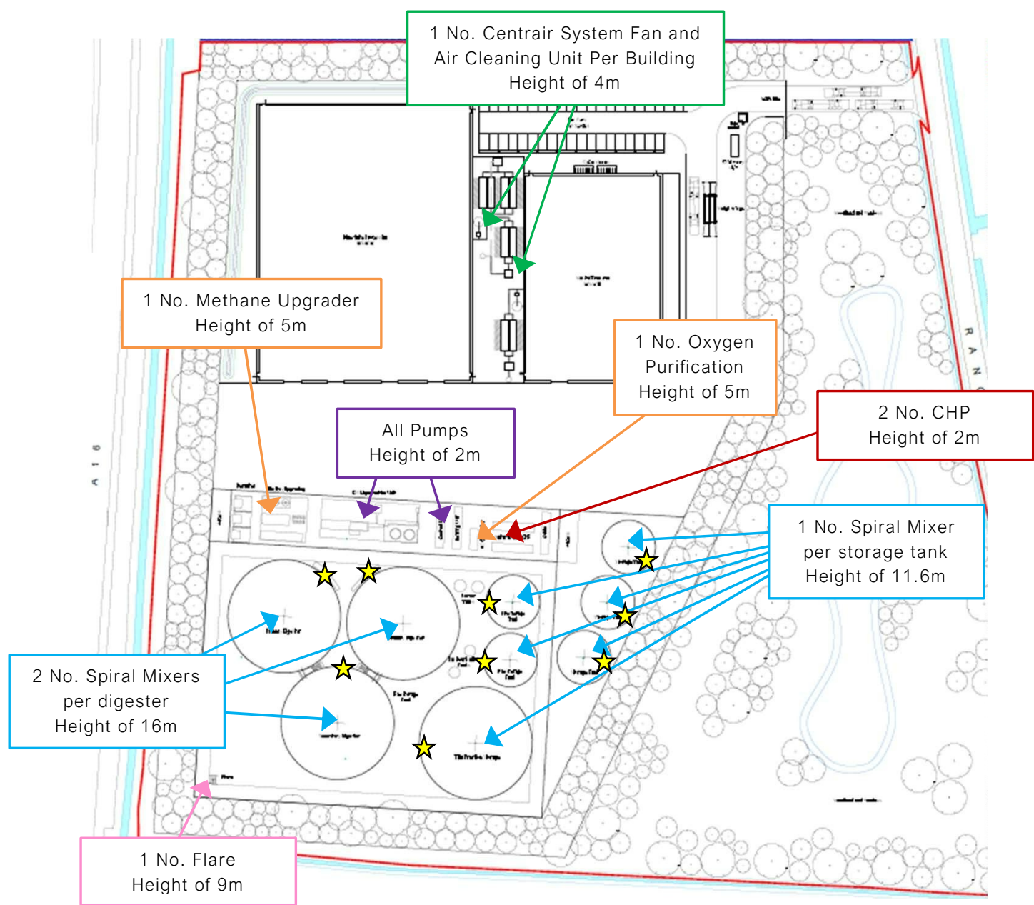
Figure 5 – Assumed Plant Locations
