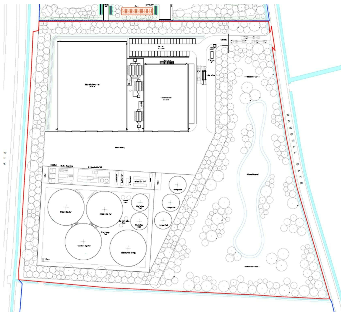
Figure 1 – Site Layout Plan of Proposed Development
