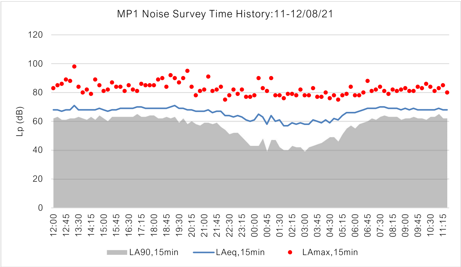
Figure 10 – MP1 Noise Survey Time History
