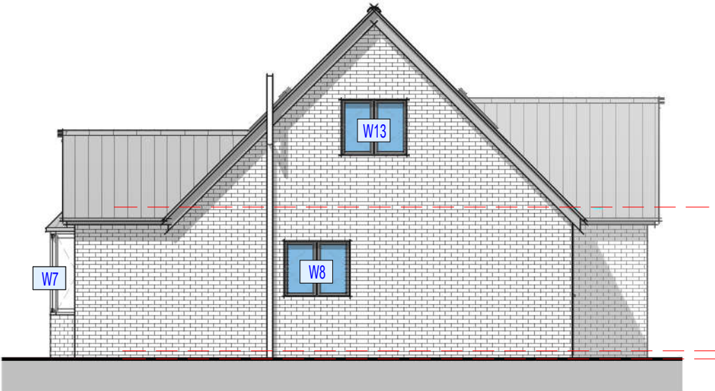
Elevation 02 - Right (west)
