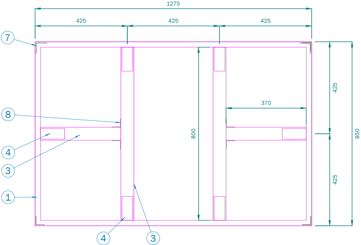
FRAMEWORK SCALE 1:10
