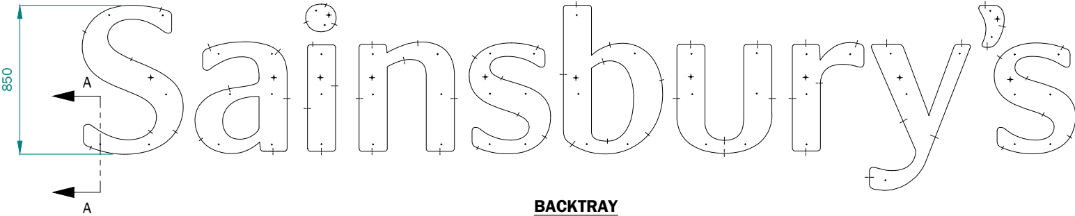
BACKTRAY SCALE 1:30
