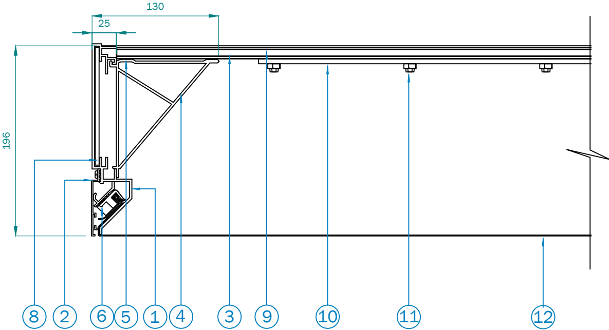
PARTIAL BROKEN SECTION SCALE 1:4
