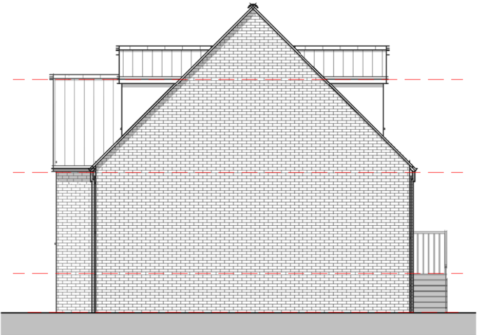
Elevation 02 – Right 1 : 100
