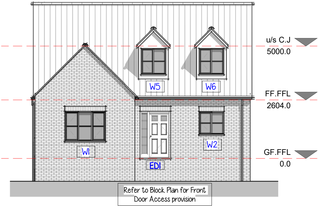
Elevation 01 – Front 1 : 100
