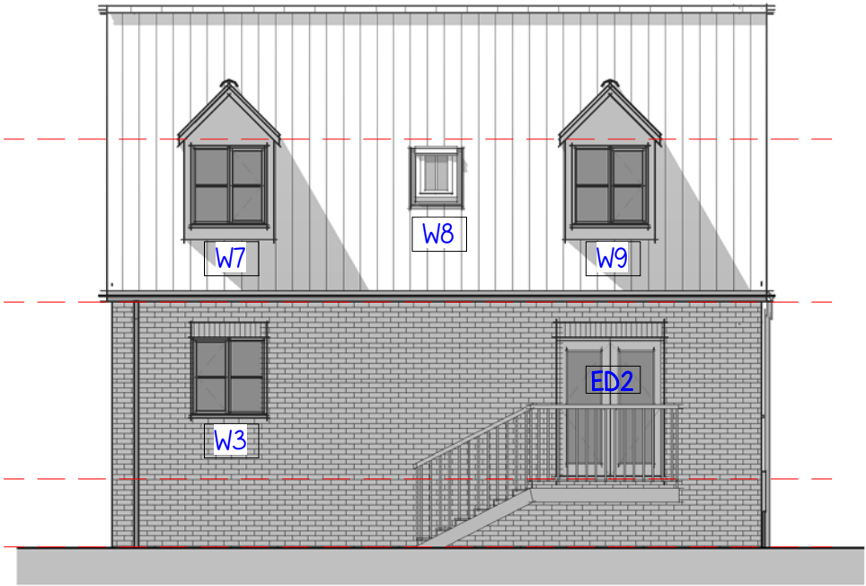
Elevation 03 – Rear 1 : 100
