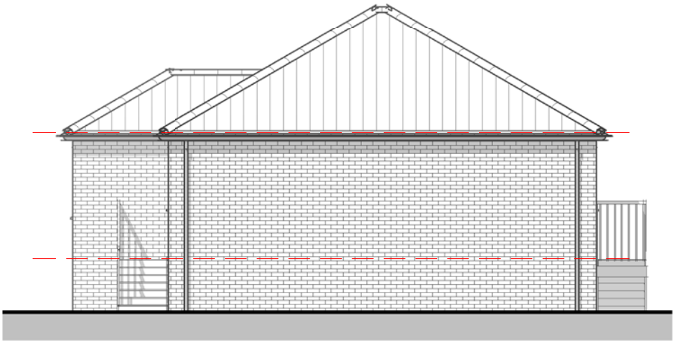
Elevation 02 – Right 1 : 100
