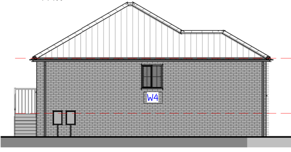
Elevation 04 – Left 1 : 100
