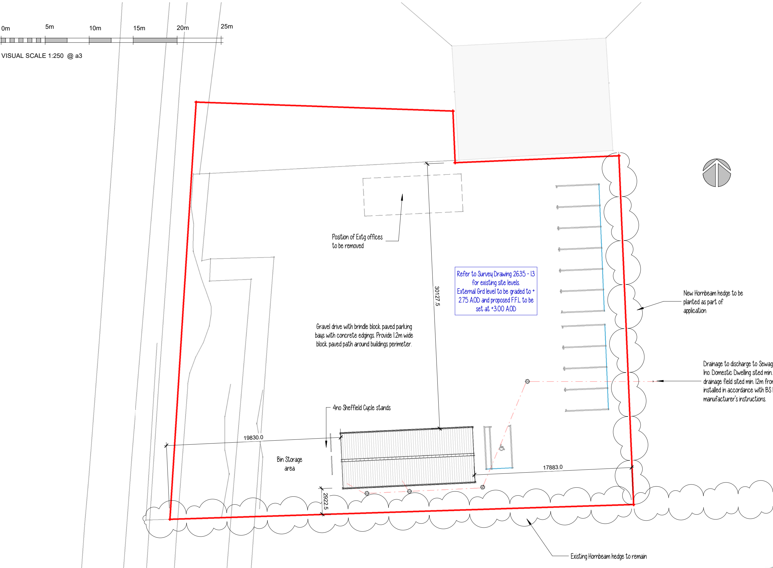
Site Block Plan
