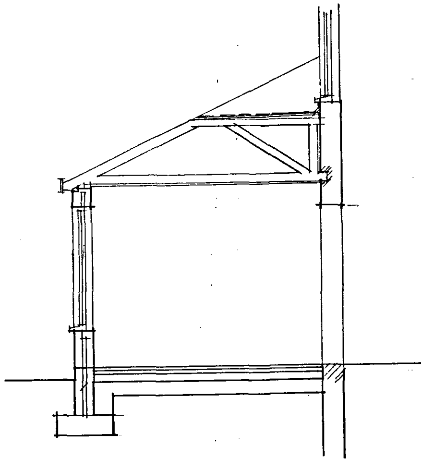
SECTION
