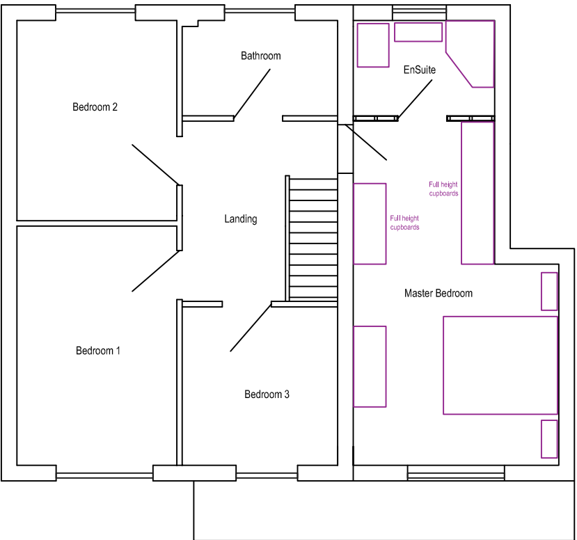
Proposed layout to First Floor
