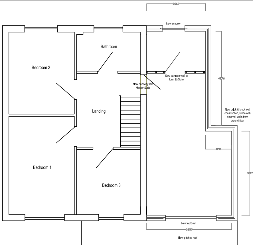
Proposed alterations to First Floor
