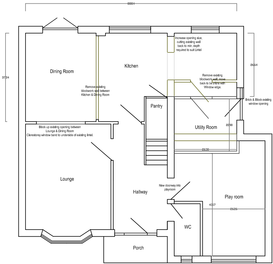
Proposed alterations Option 2
