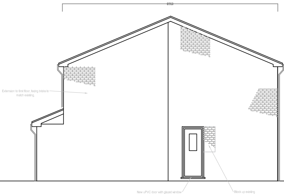
Proposed Side Elevation Option 2
