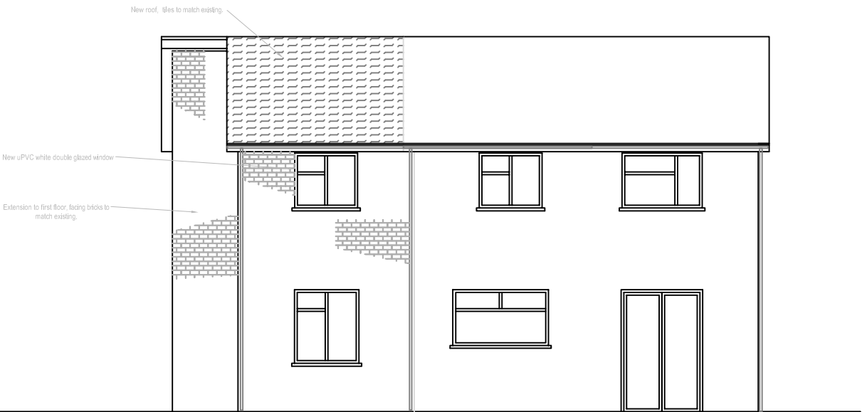
Proposed Rear Elevation Option 2
