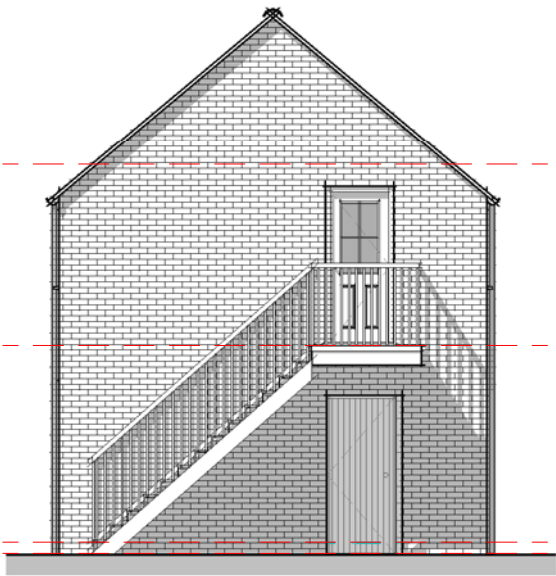
Elevation 02 – Right 1 : 100
