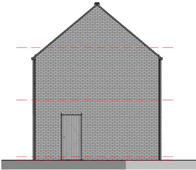
Elevation 04 – Left 1 : 100
