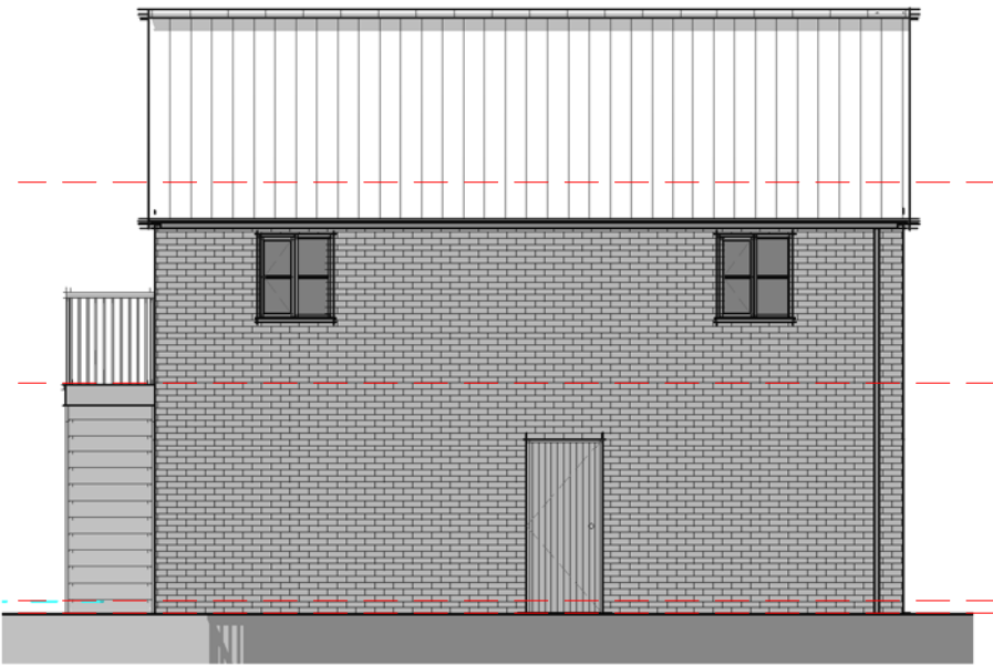
Elevation 03 – Rear 1 : 100
