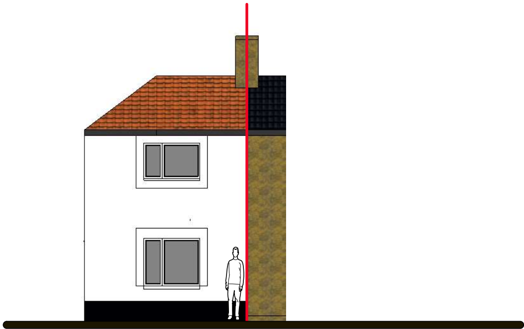
A 3 Rear Elevation 1:100
