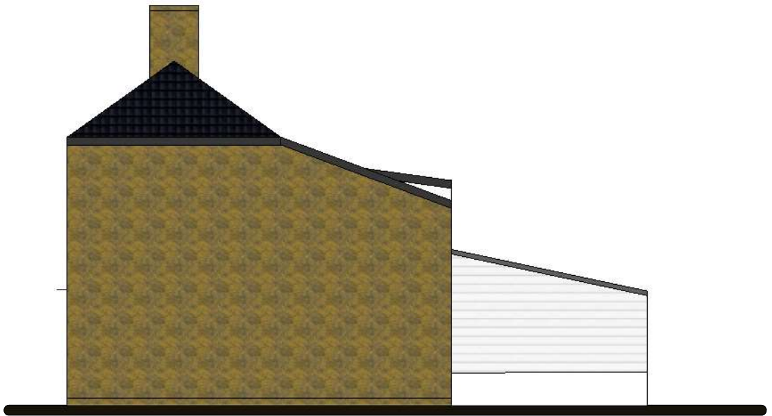
A 6 Side Elevation 1:100
