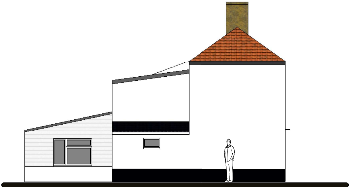
A 4 Side Elevation 1:100
