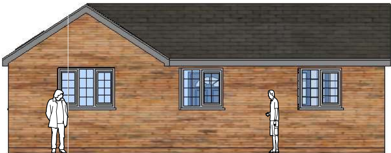
A 15 Rear Elevation 1:100
