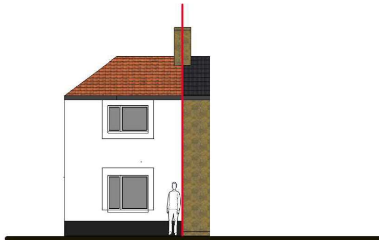
A 5 Front Elevation 1:100
