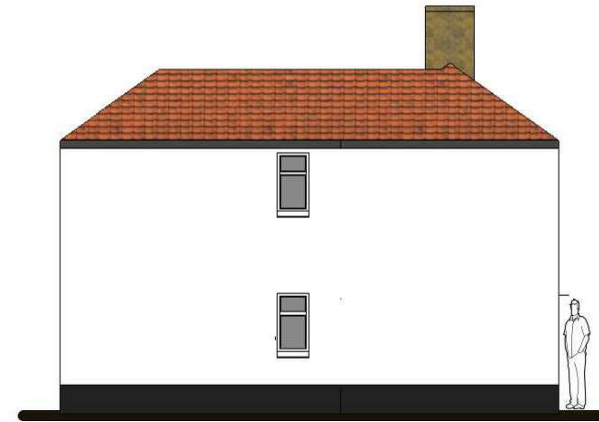
A 10 Side Elevation 1:100
