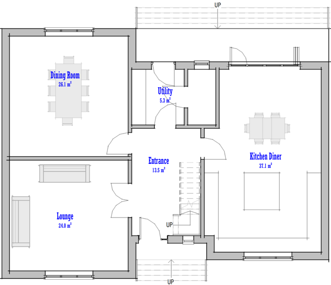
Plan 01 - Ground 1 : 100
