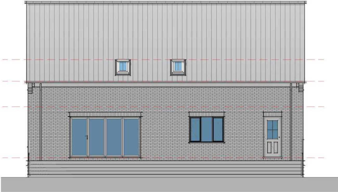
03 Elevation - Rear
