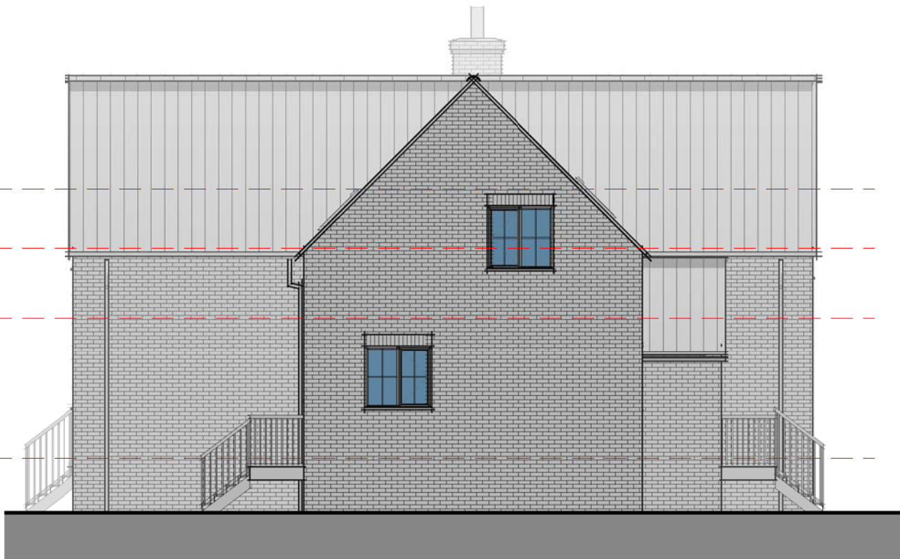
Elevation 04 - Left
