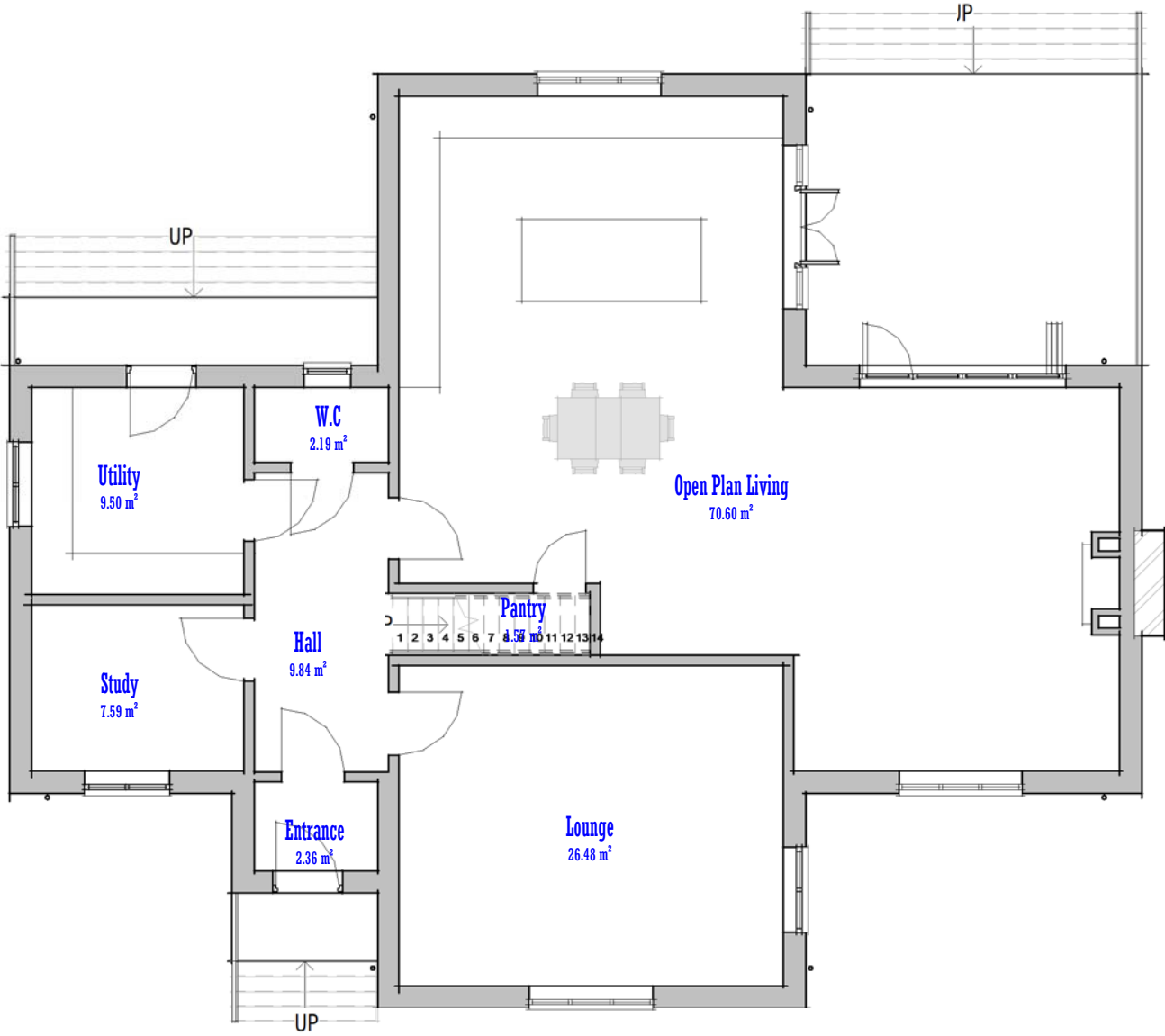
Plan 01 - Ground 1 : 100
