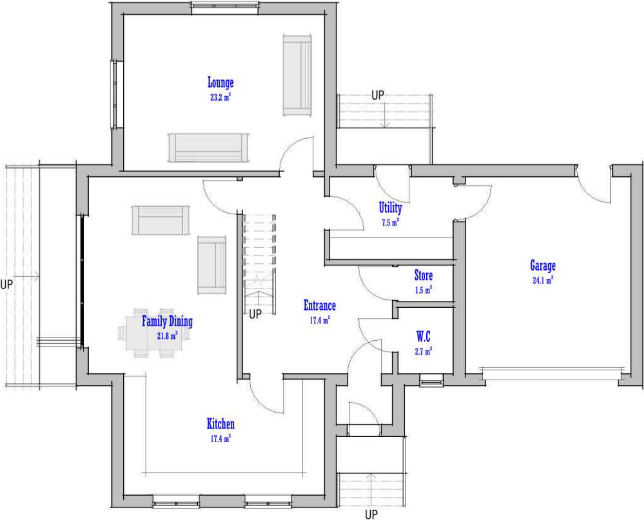
Plan 01 - Ground 1 : 100
