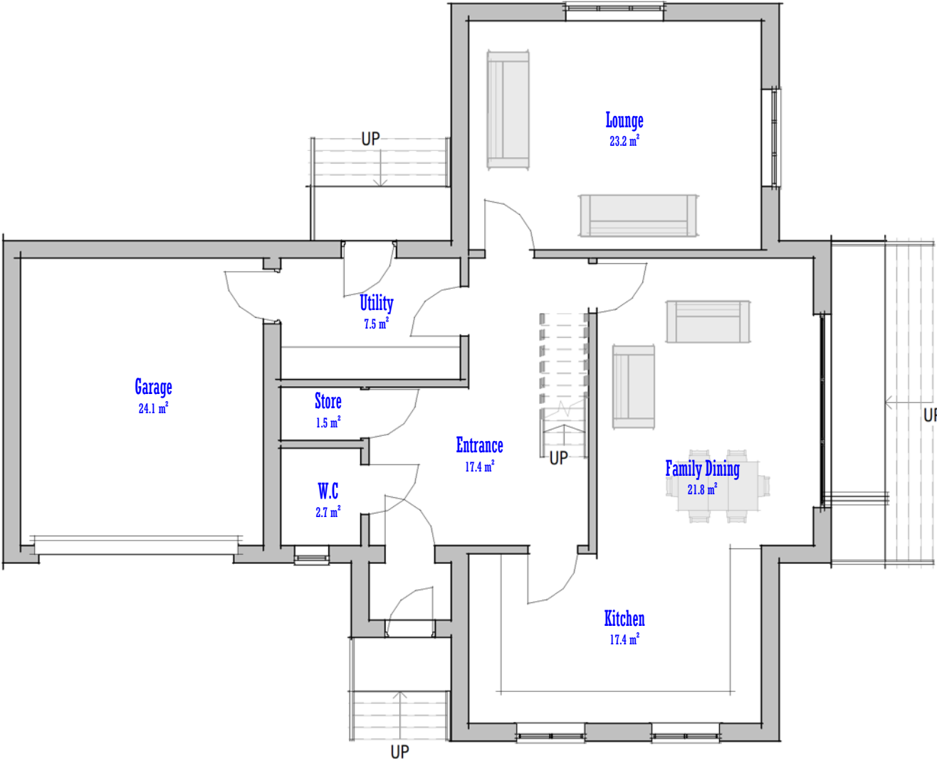
Plan 01 - Ground 1 : 100
