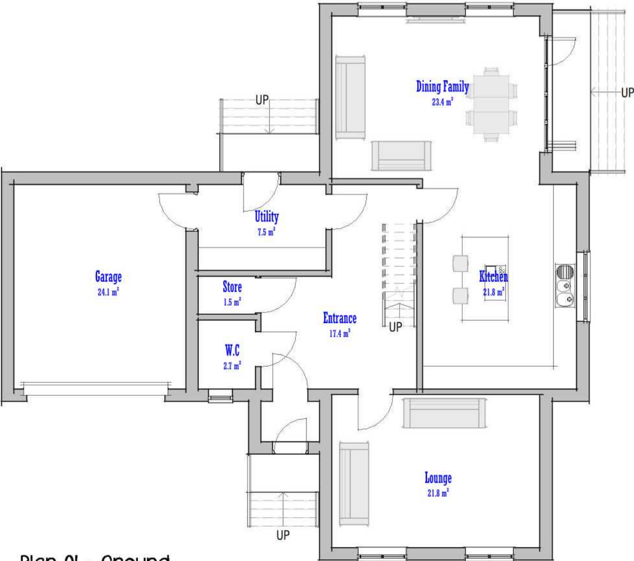
Plan 01 - Ground 1 : 100
