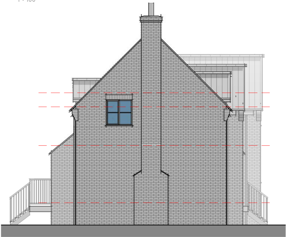
Elevation 04 - Left
