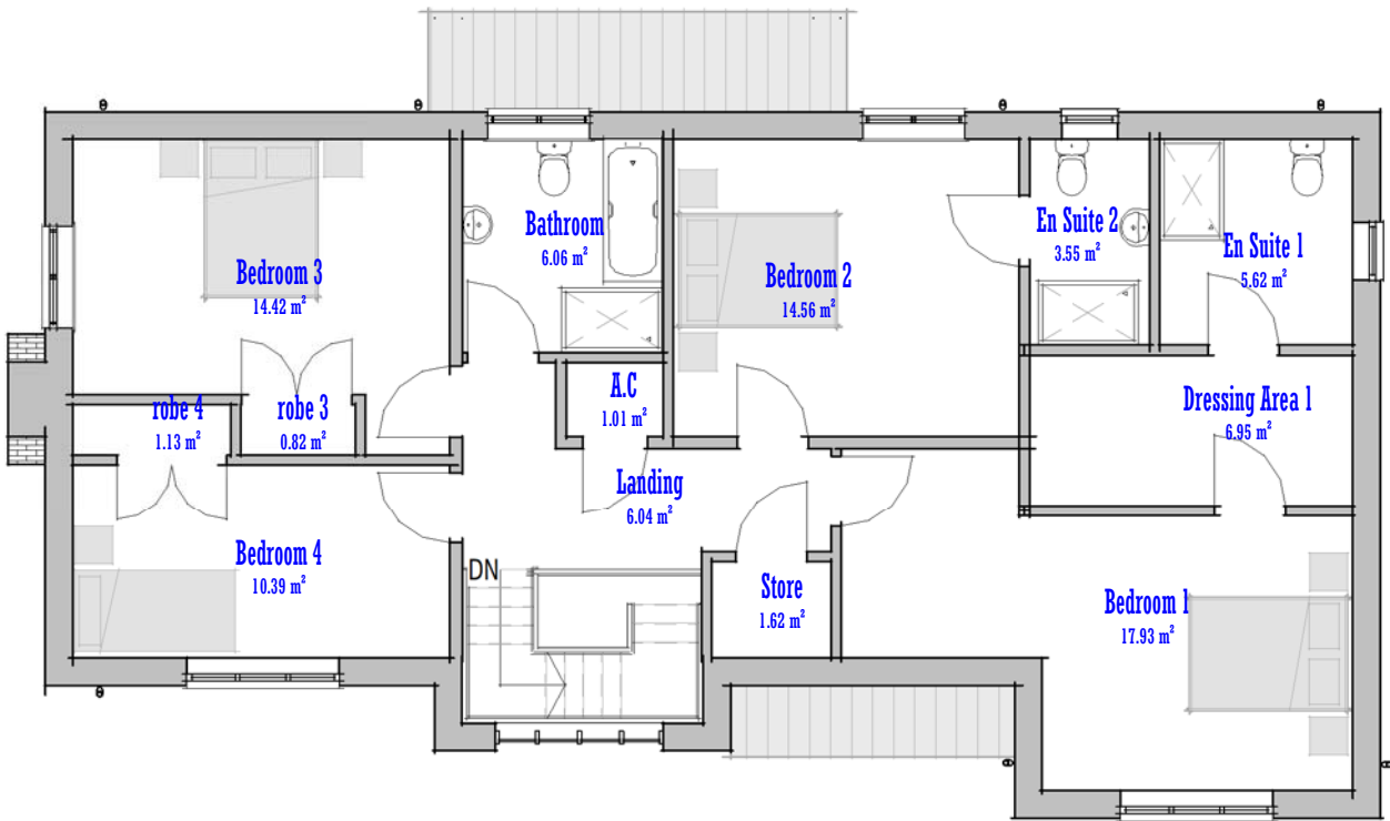
Plan 02 - 1st Floor Plan
