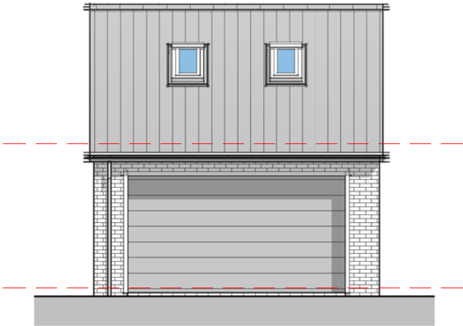
Elevation 01 - Front 1 : 100
