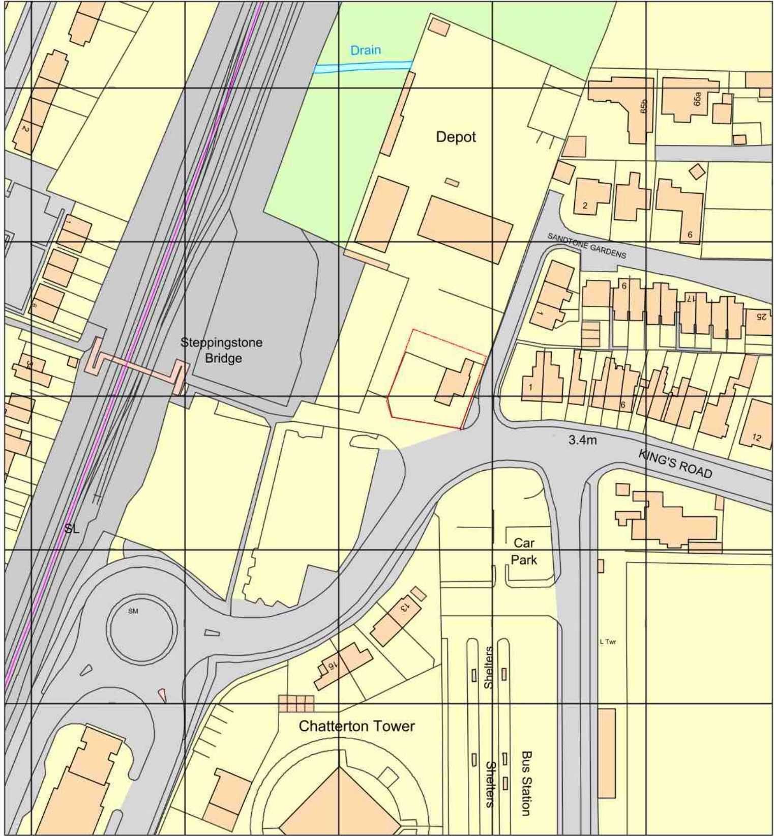
EXISTING SITE LOCATION PLAN Scale 1:1250
