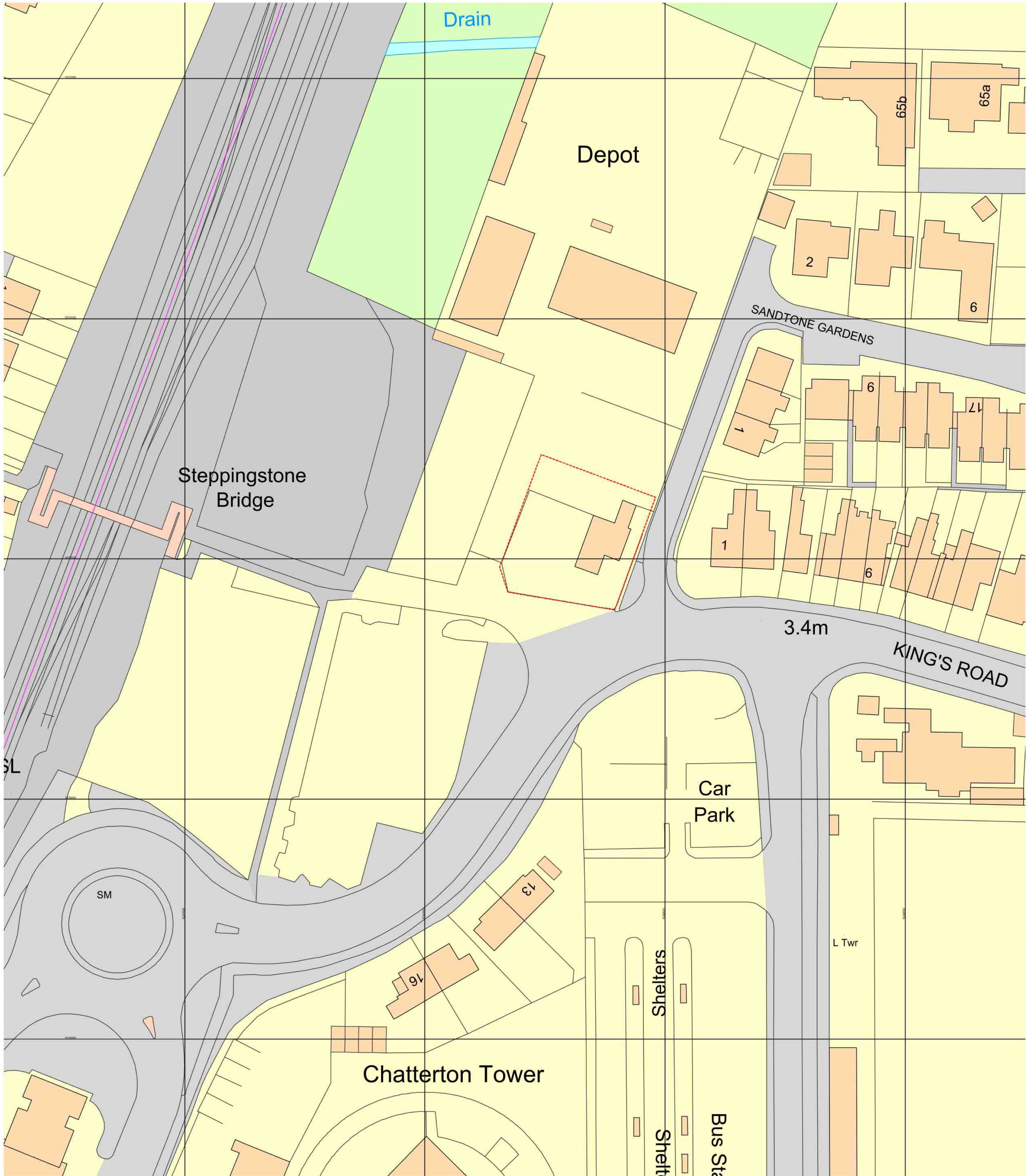
EXISTING SITE BLOCK PLAN Scale 1:500
