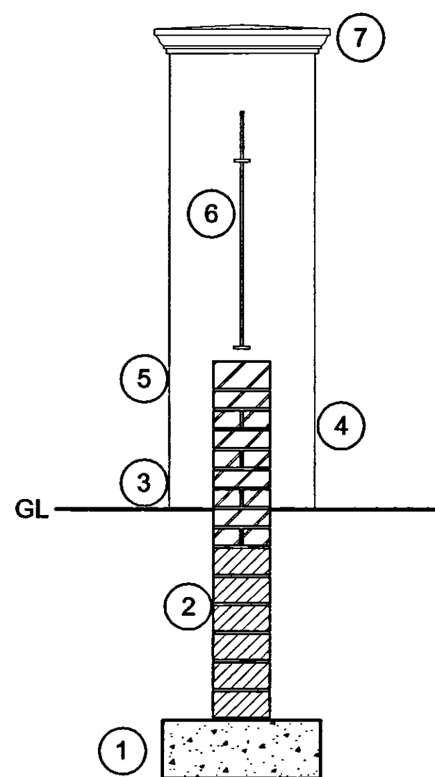
Typical Section 1:20
