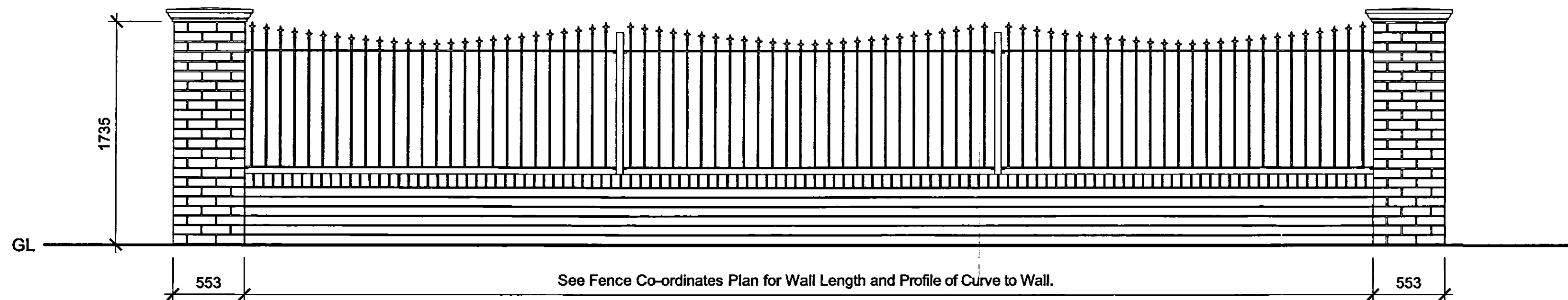
Typical Elevation of Wall (not to scale)
