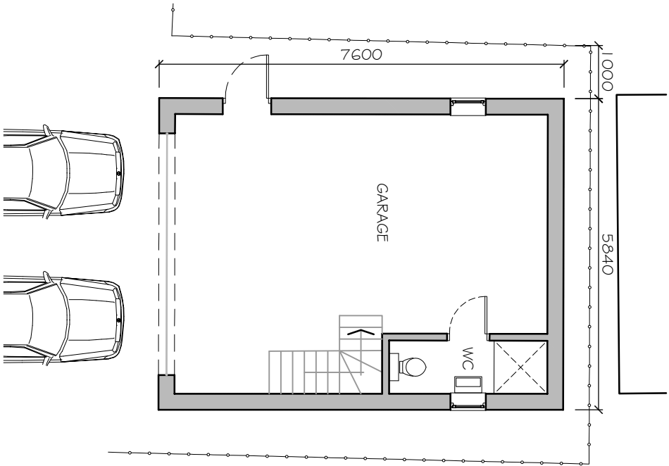
PROPOSED GROUND FLOOR GA PLAN.
