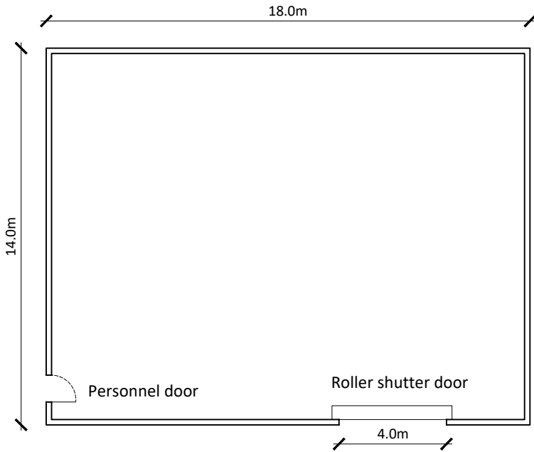
FLOOR PLAN
