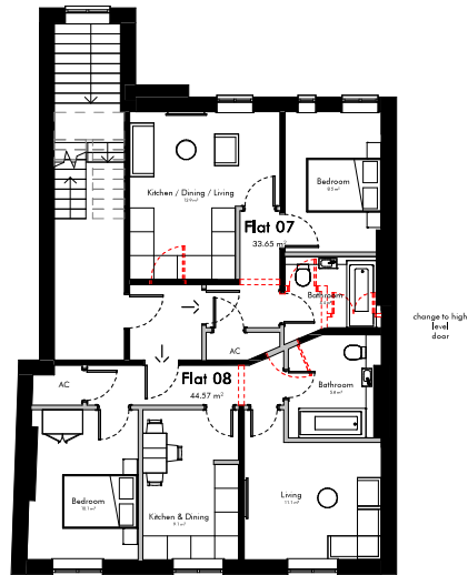
Level 02 - Second Floor- Proposed
