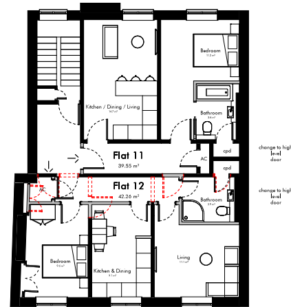
Level 04 - Fourth Floor - Proposed
