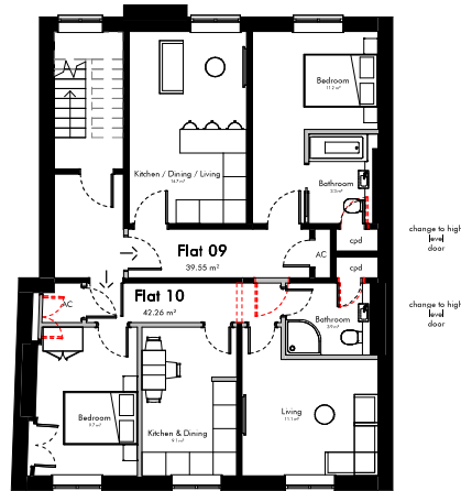
Level 03 - Third Floor - Proposed
