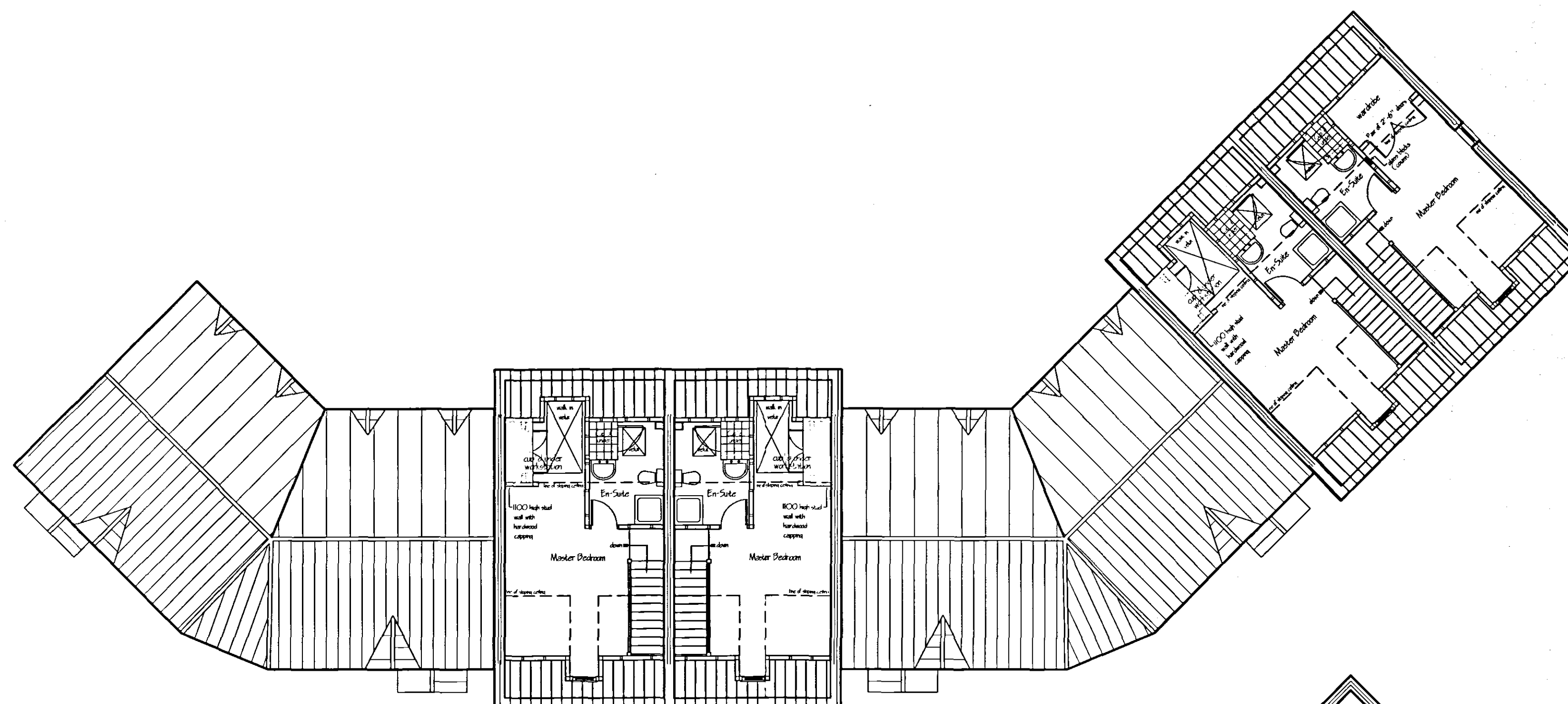
SECOND FLOOR LAYOUT
