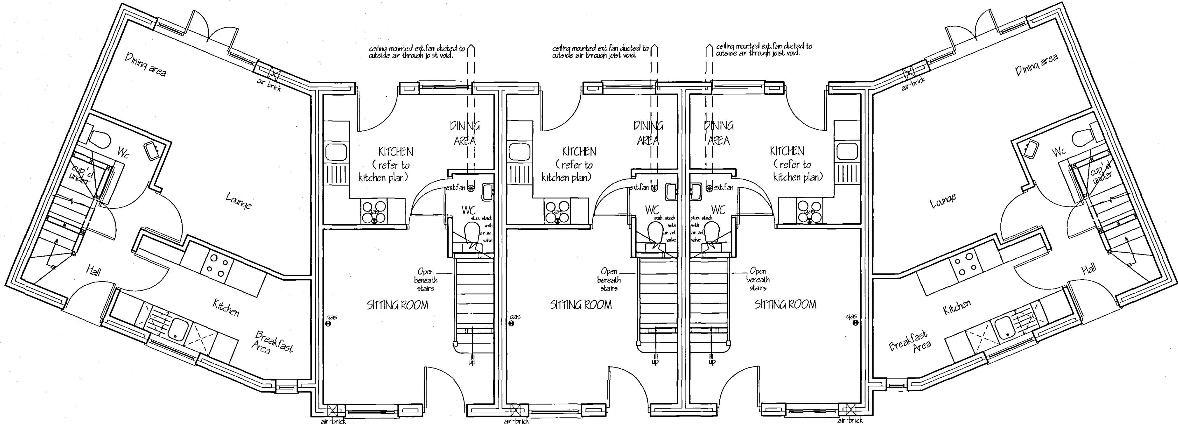
GROUND FLOOR LAYOUT
