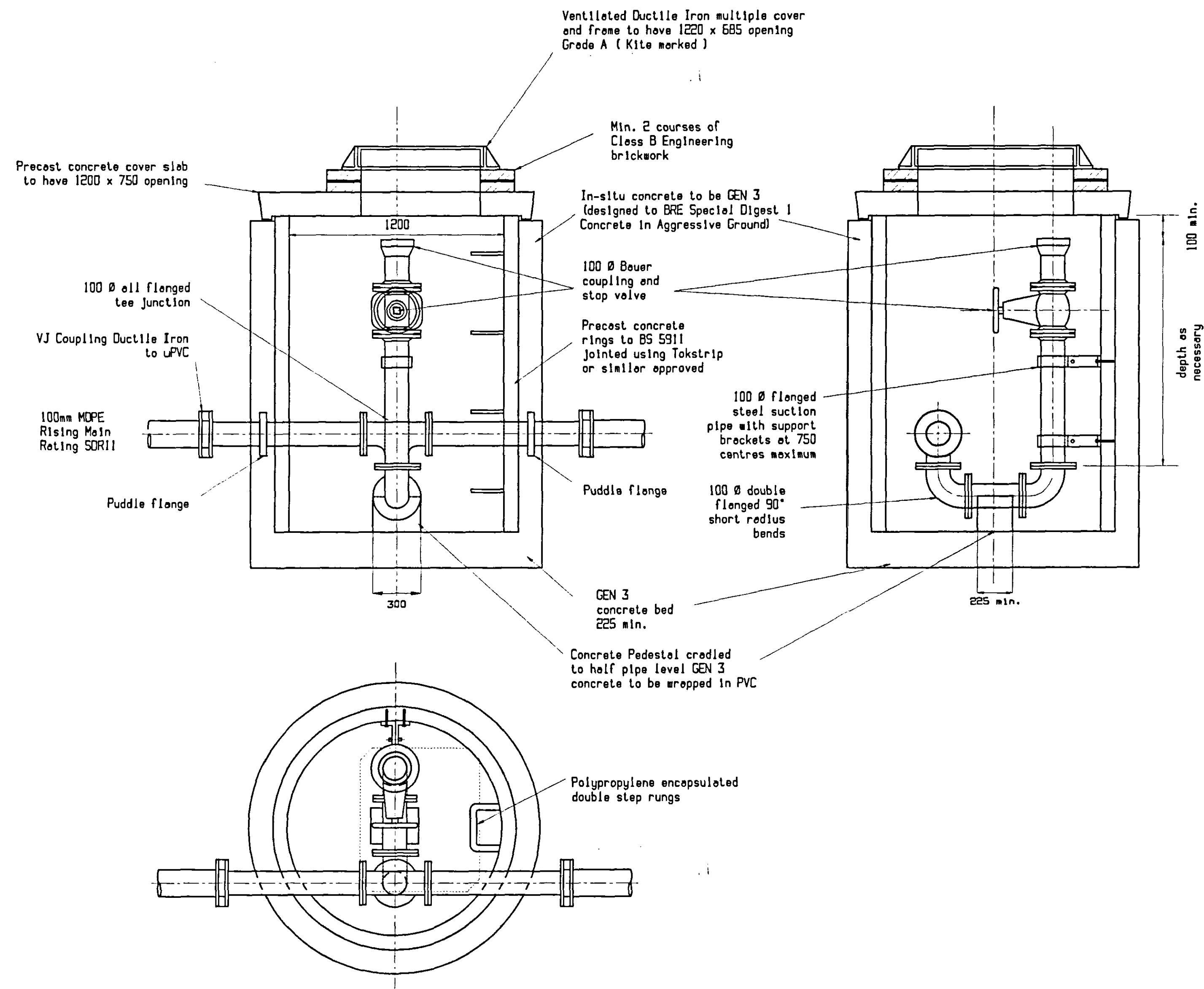
STANDARD WASH OUT VALVE DETAIL
