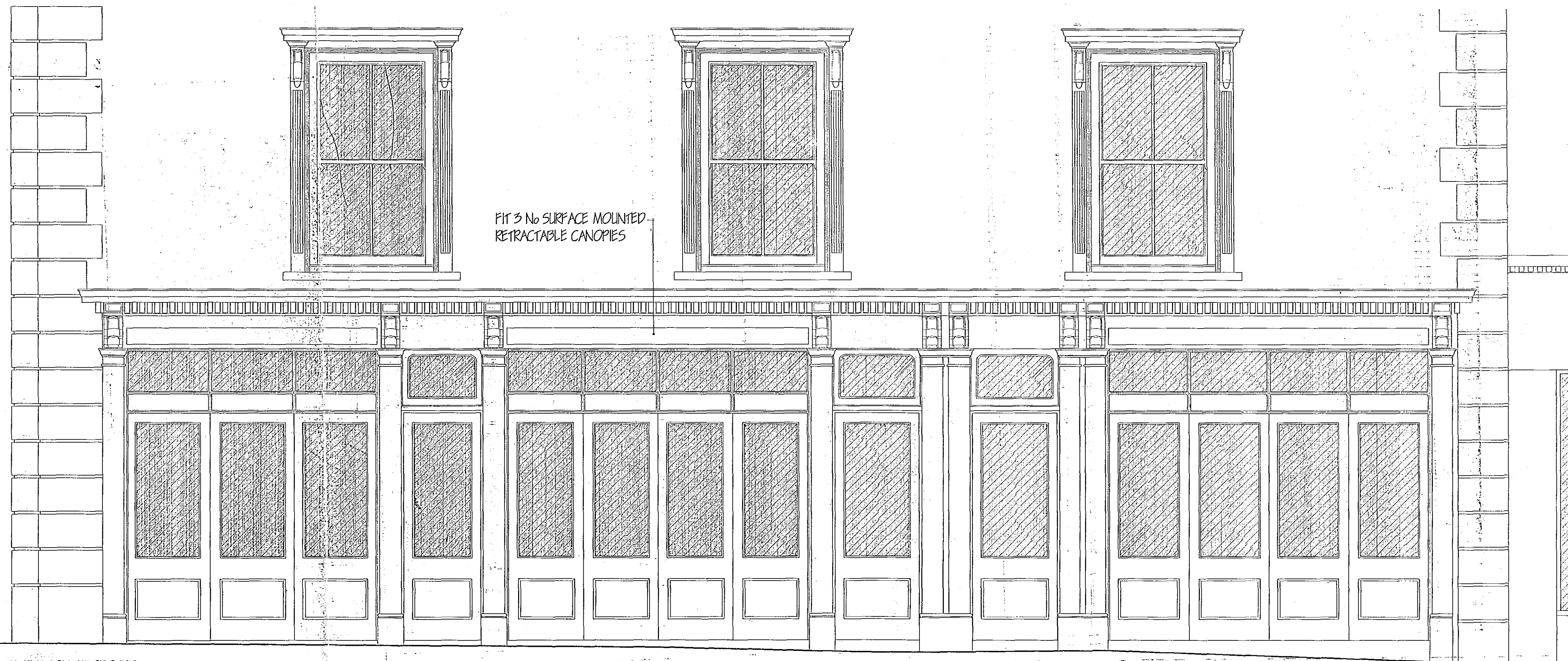
ELEVATION PROPOSED
