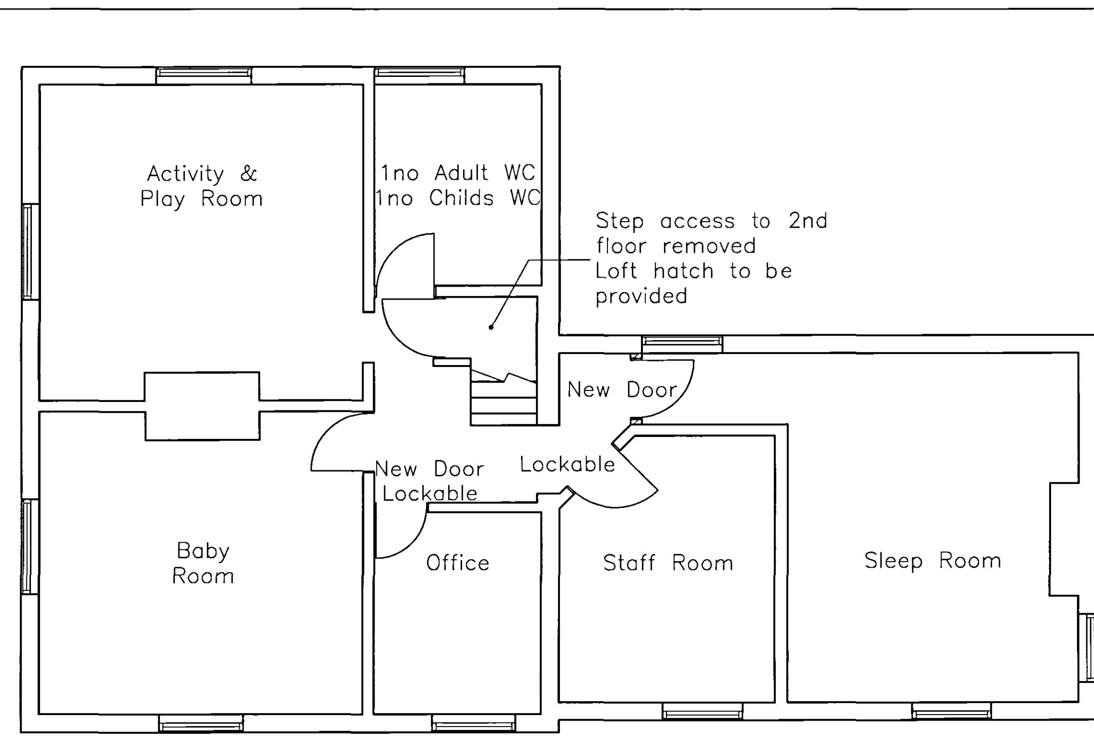
First Floor
