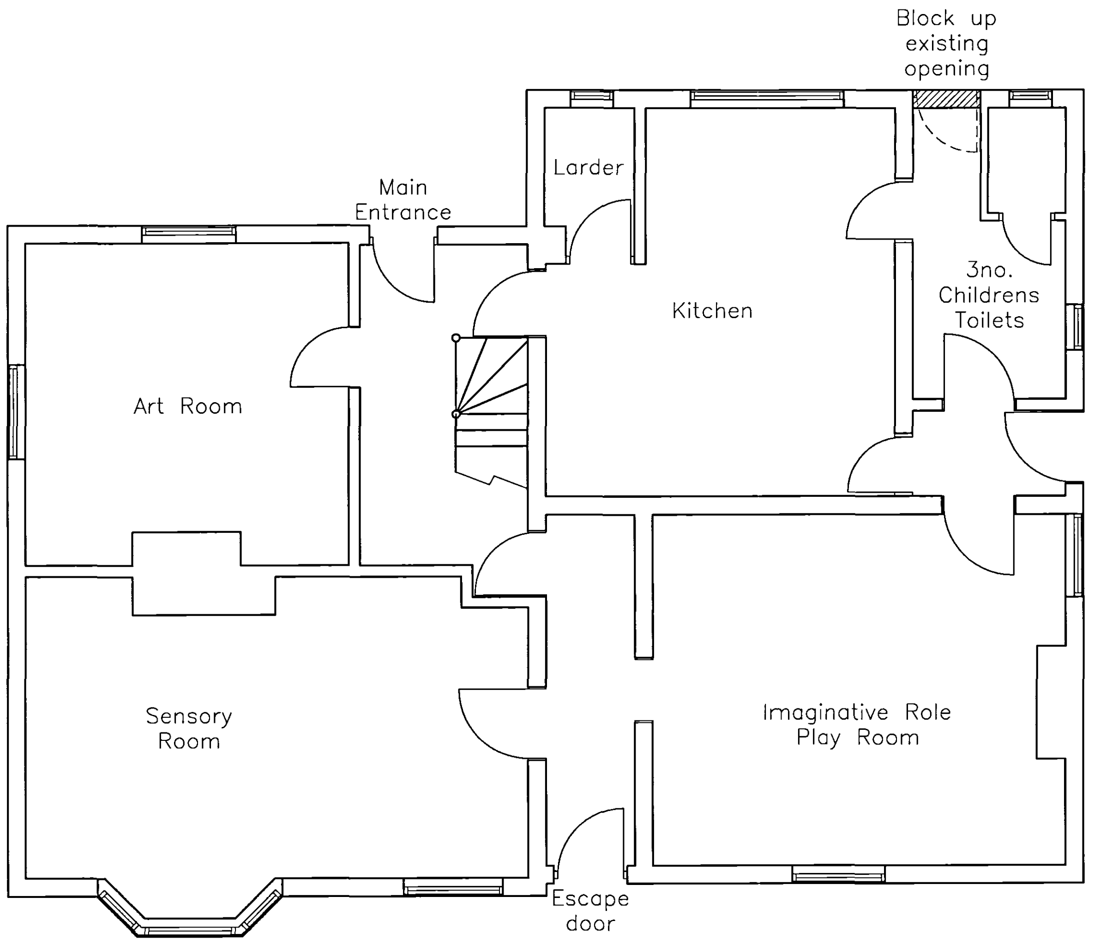
Ground Floor
