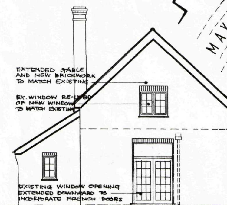
REAR ELEVATION
